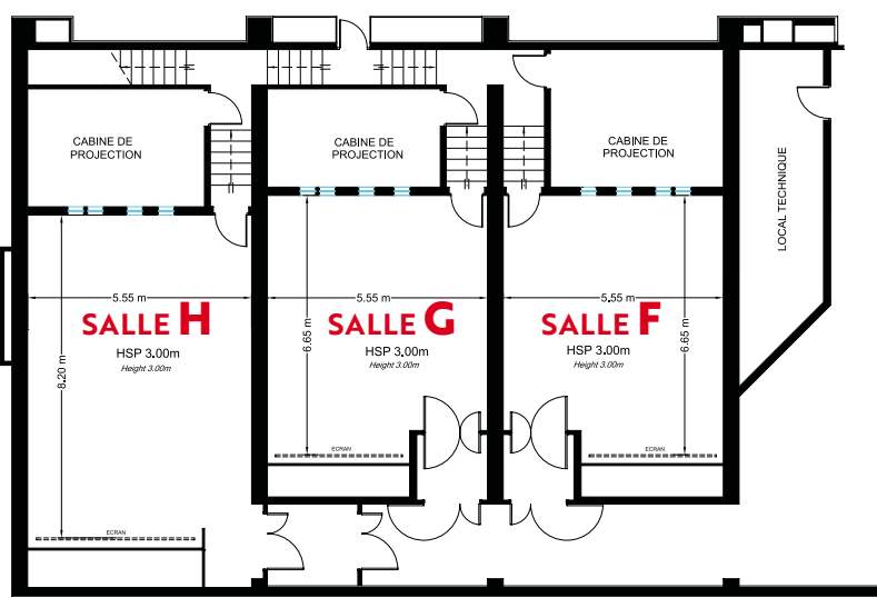
GENERAL PLAN
